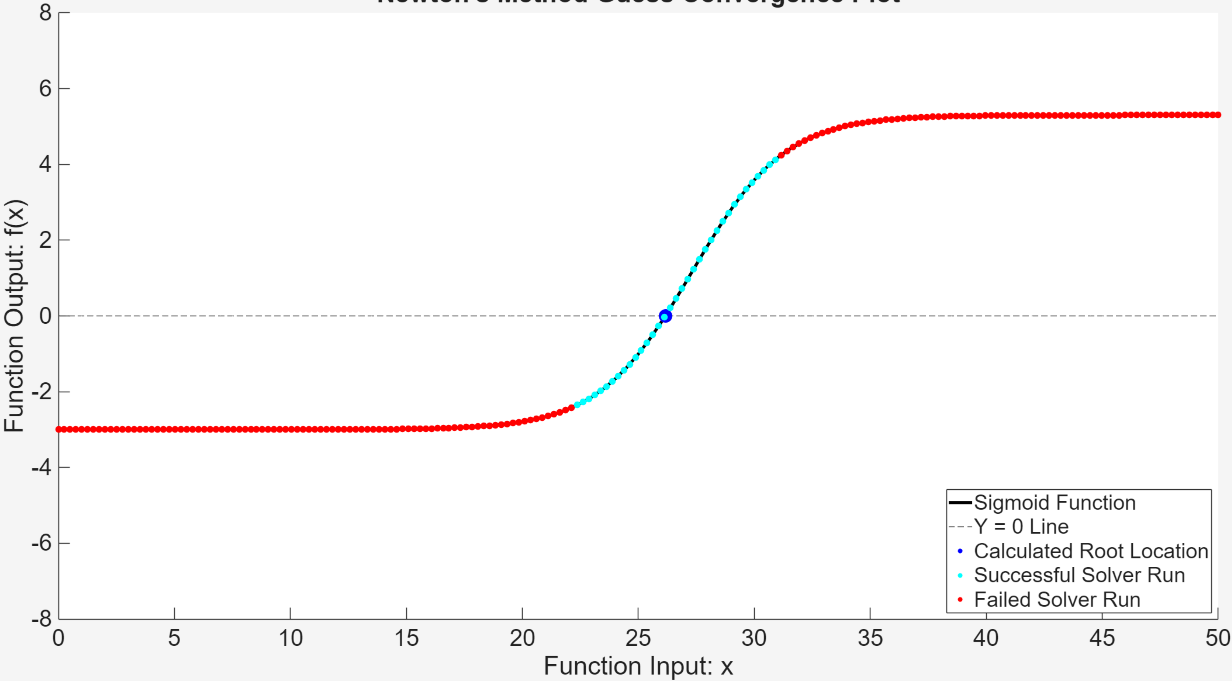
Newton's Method Guess Convergence Plot
